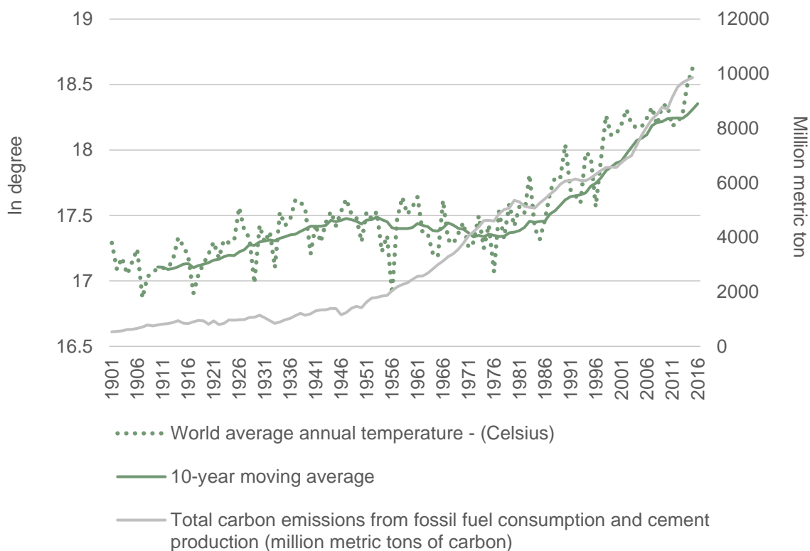
Chart 2: Temperature Increase and Carbon Emissions
