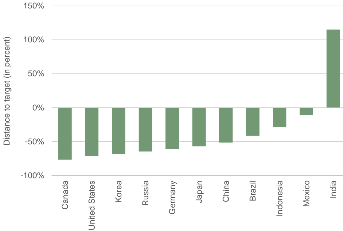
Chart 3: 2015 GHG Emissions Distance to Target (2030)
